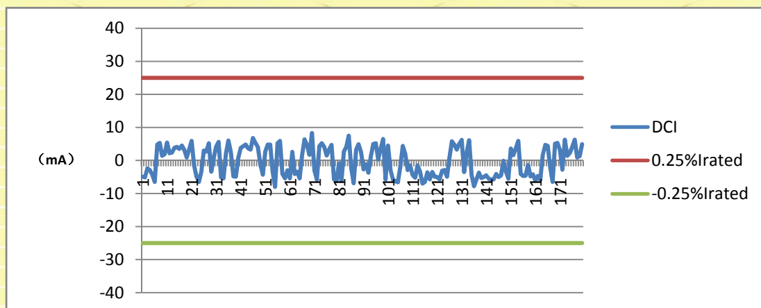
Diagramm of permanent DC-Injec
